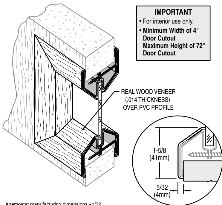
Dimensions for Wood Veneers
